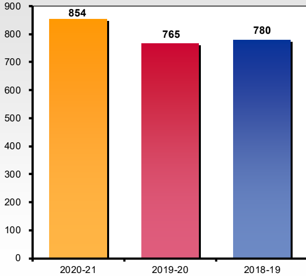
Heating Degree Days--YTD September - October
